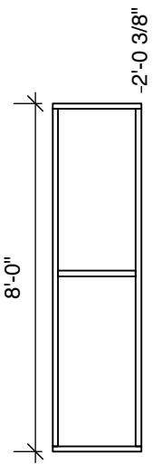
Frame 15 - 2" x 6"
