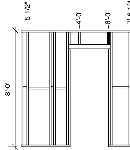
Frame 7 - 2" x 6"
