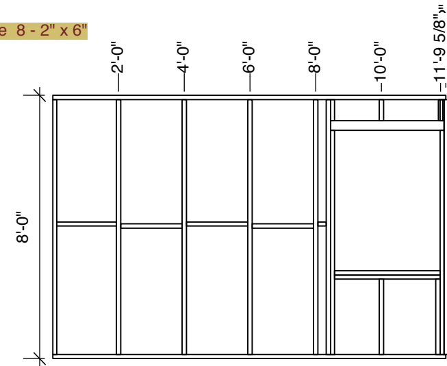
Frame 4 - 2" x 6"
