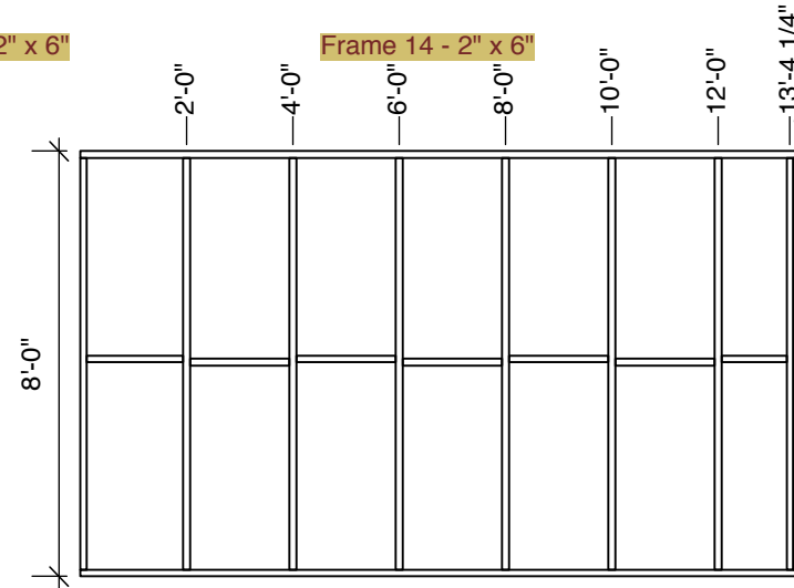
Frame 8 - 2" x 6"
