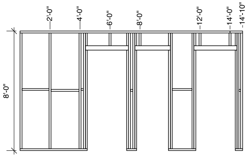
Frame 12 - 2" x 6"
