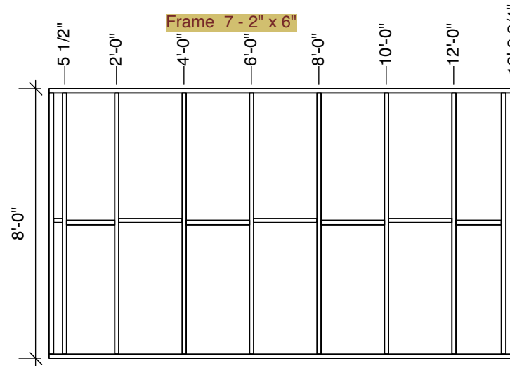
Frame 3 - 2" x 6"
