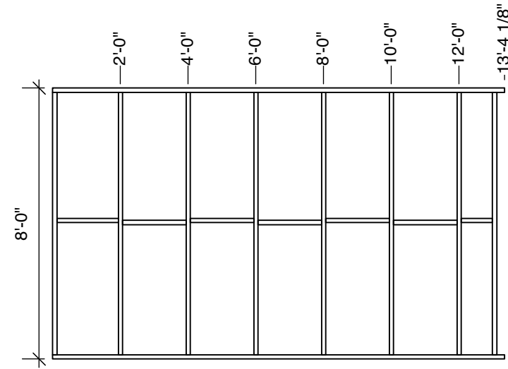
Frame 14 - 2" x 6"
