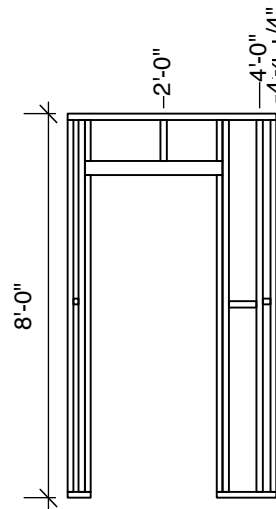
Frame 13 - 2" x 6"
