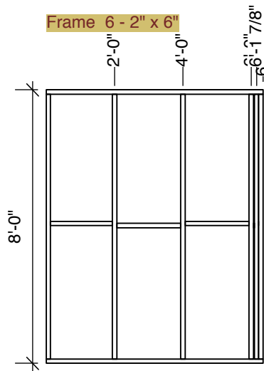
Frame 1 - 2" x 6"
