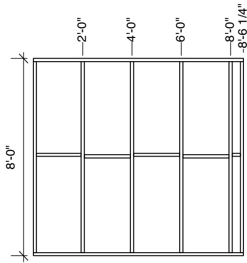
Frame 11 - 2" x 6"
